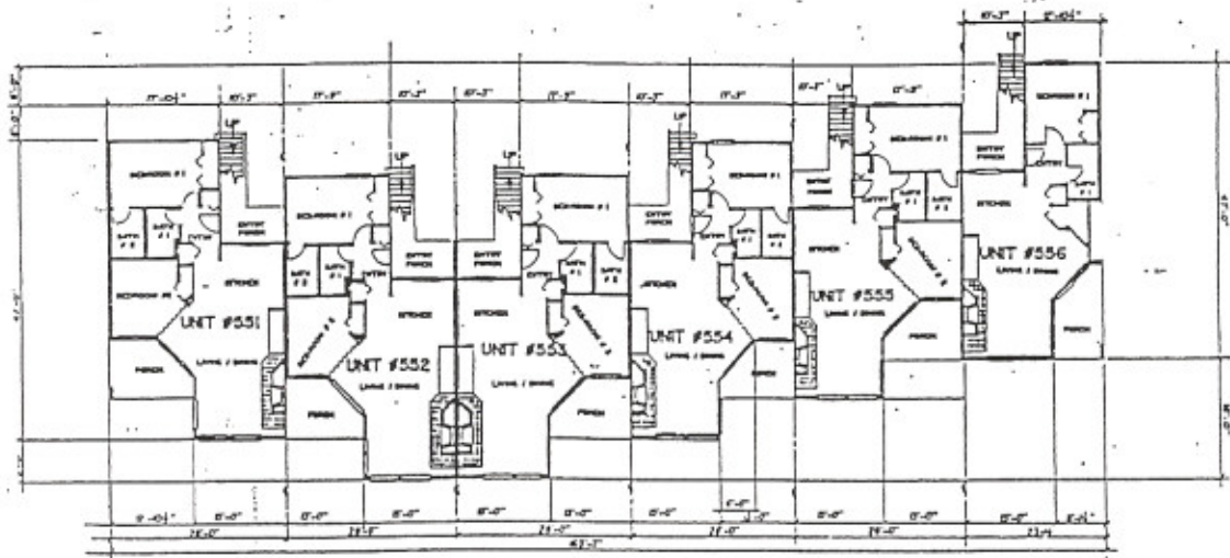
MAIN FLOOR PLAN BLDG. #3
